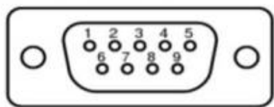
Connector Pinout
